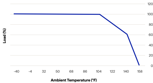
Derating Curve
